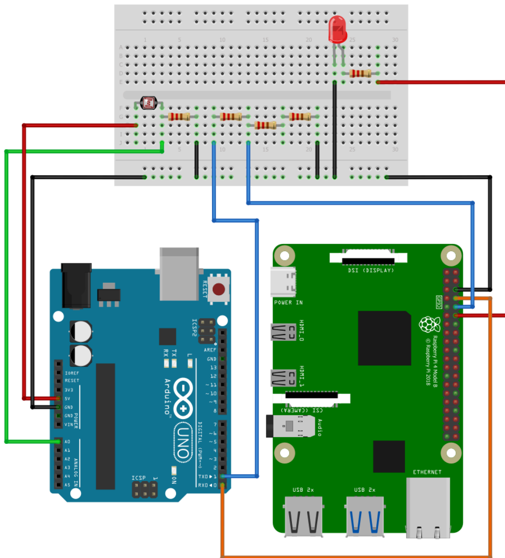
Fig. Arduino and Raspberry PI interfacing
